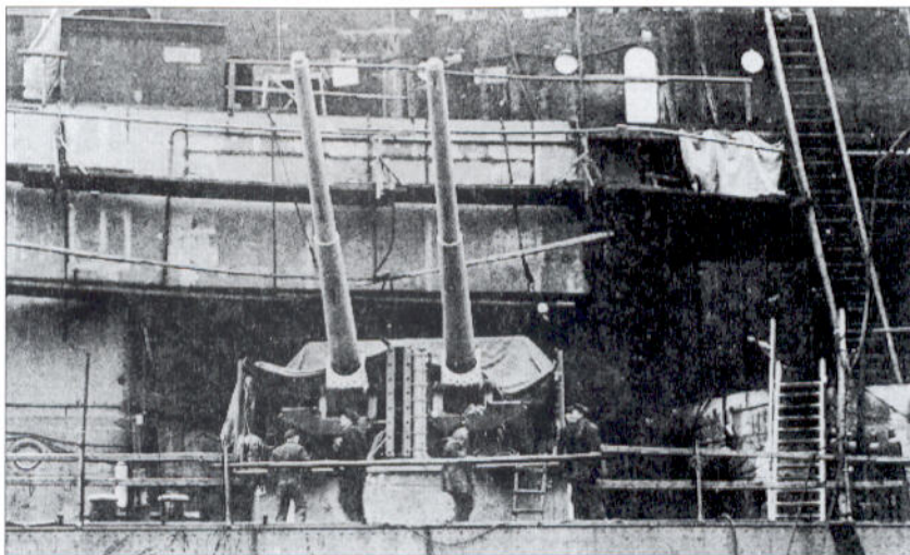
Construction of one of Bismarck's 10.5cm twin heavy flak guns. Note how the barrels are first installed on the base mount, and then the turret housing built around them.
