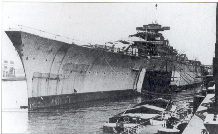
Bismarck during fitting out. The straight stem originally fitted has already been replaced by the 'Atlantic' bow.
