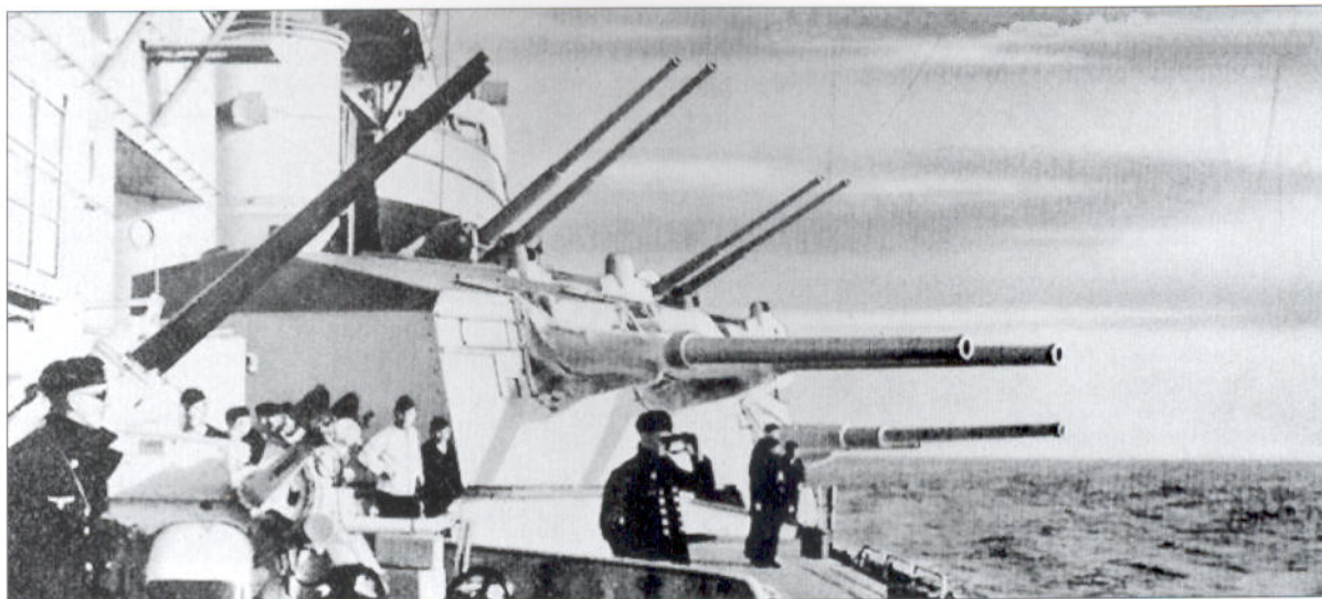
An excellent view of one of Scharnhorst 's secondary turrets, mounting 15cm guns. The guns shown at high elevation behind this turret are those of her main 10.5cm flak batteries. One of the ship's boats can be seen just above these flak guns.
