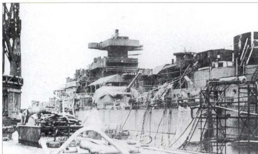
Bearing little resemblance to the sleek, graceful ship she would soon become, Bismarck is covered with clutter and liberally draped with electrical cabling to power the workers' tools and provide lighting to the ship's interior. The roofed structure just visible above the secondary turret is the port hangar for the ship's Arado 196 floatplanes.
