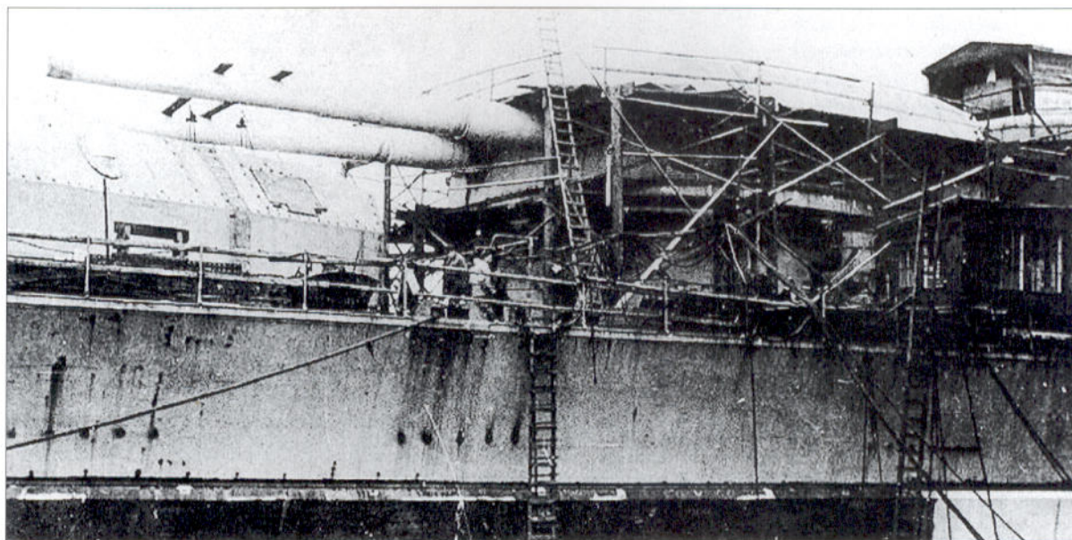
Construction of the main 38cm gun turret 'Bruno' during fitting out. The guns are in place and work is ongoing in building the armoured turret around them. The plethora of scaffolding and ladders is typical of a ship under construction.
