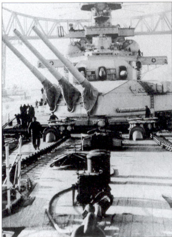
The view towards the forward turrets 'Anton' and 'Bruno' from the bow of Scharnhorst , gives a good impression of the huge size of her main armament. Note that the canvas blast bags are fitted on the gun barrels of turret 'Anton' only. This shot also gives a good view of the large searchlight mounted on the face of her tower just above the bridge.
