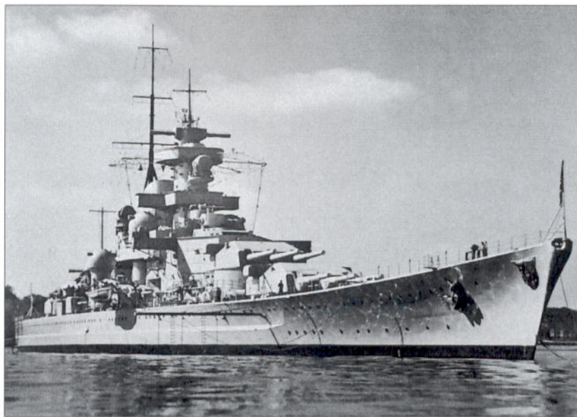
This view shows Gneisenau after her refit, now sporting the raked 'Atlantic' bow, which did little to cure her tendency to ship considerable amounts of water over her fo'c'sle at speed or in heavy seas. The angled funnel cap can just be seen by the base of her mainmast. That this is a pre-war photograph is confirmed by the presence of the ship's crest on the bow. It was removed on the outbreak of war.
