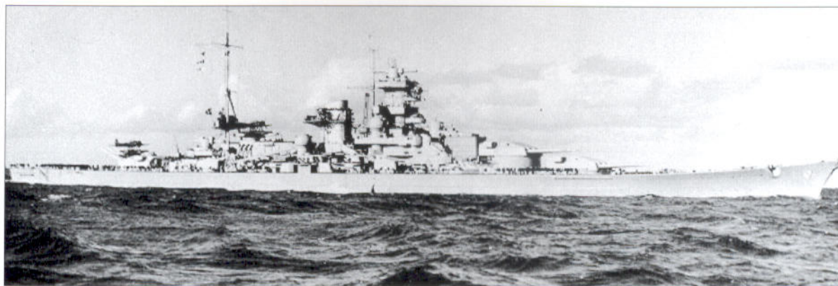
Scharnhorst in post-refit form with 'Atlantic' bow and angled funnel cap, but still retaining the second aircraft catapult on turret 'Caesar'. Although very similar to Gneisenau, her identity is immediately established by the siting of the mainmast, which on Gneisenau remained sited to the rear of the funnel.
